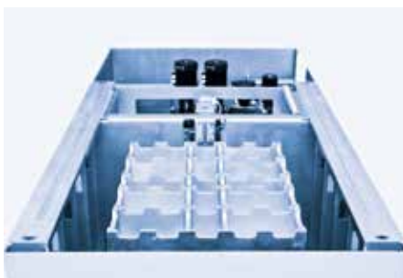
Machine bed as welded construction Grouted with mineral cast.
